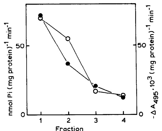
Fig.5. Specific activities of non-latent K^+, Mg^{2+} -ATPase (○) and initial rates of H^+ -pumping (●) (data from figs 2 and 4, respectively).
