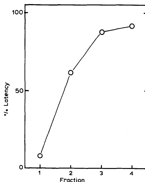
Fig.3. Latency of the K^+, Mg^{2+} -ATPase activity. The latency was calculated from the data in fig.2 as:
