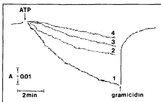
Fig.4. Proton pumping as measured by acridine orange absorbance decrease in fractions 1-4 obtained after counter-current distribution (fig.1). The plasma membranes used as starting material showed a H^+ -pumping similar to fraction 3. The H^+ -gradient was collapsed by 20 \mu M gramicidin in all fractions (only shown for fraction 4).
